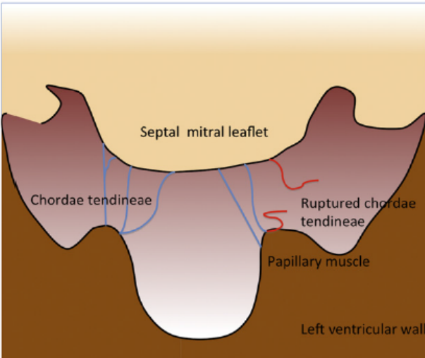
Figure 2. A schematic depicting rupture of the chords in mitral valve disease that usually tether the valve edges in place
